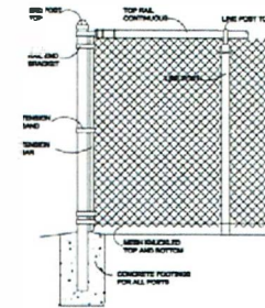
TYPICAL CHAINLINK FENCING POWDER COATED COLOUR BLACK
